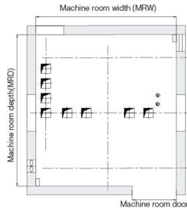
Machine Room Opening Plan
