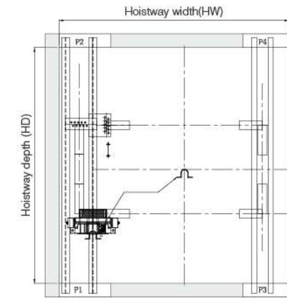
Hoistway Beam Plan
