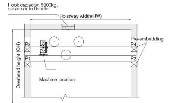
Hoistway Beam Opening Elevation
