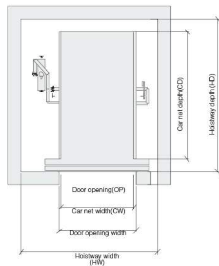
Hoistway Plan
