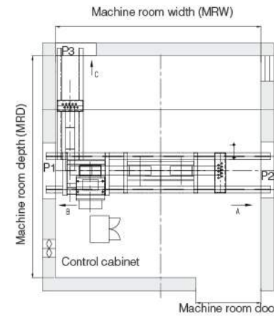
Machine Room Plan
